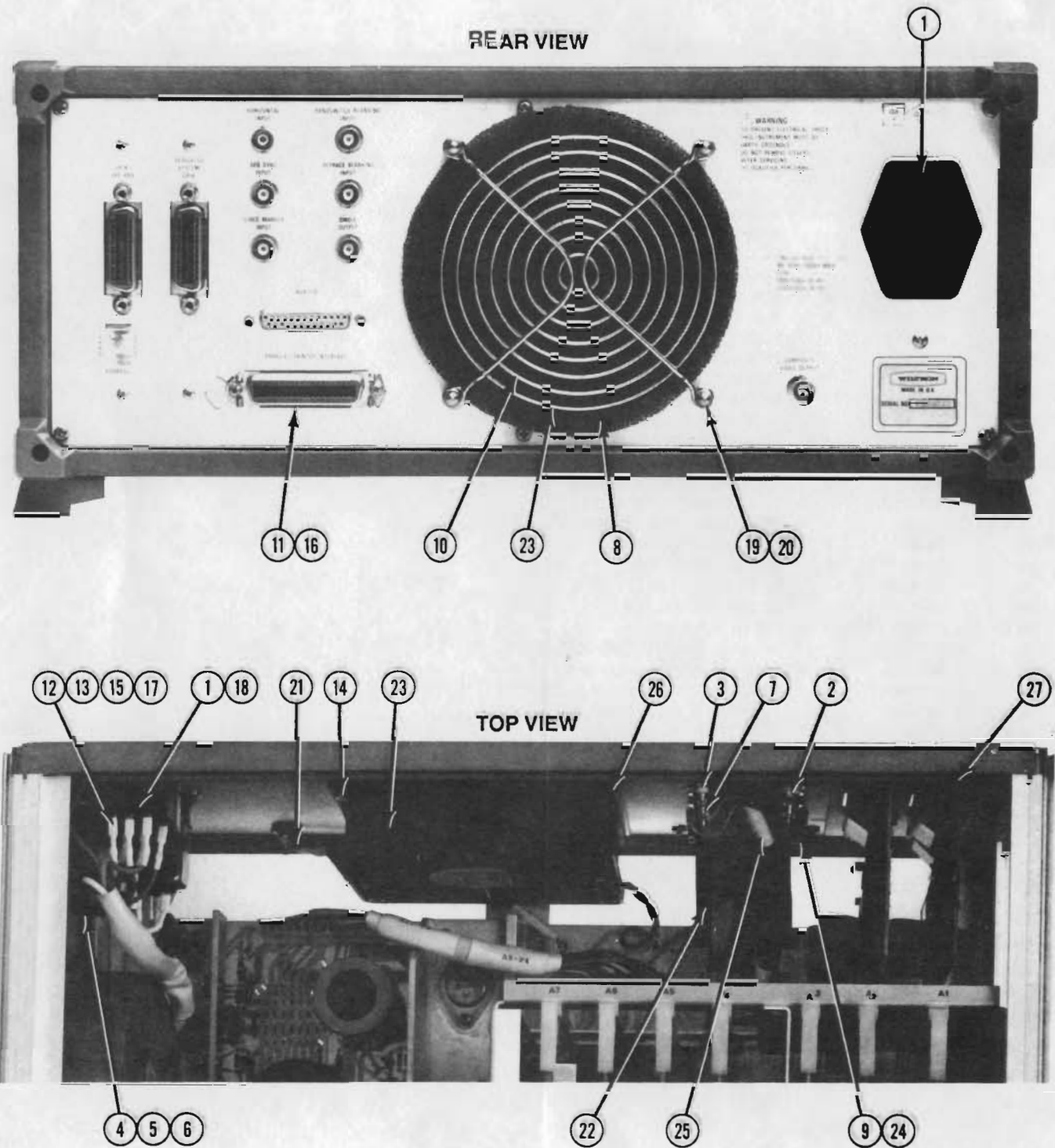
Figure 5-3. Rear Panel 561-D-32503 Sheet 1 of 1
