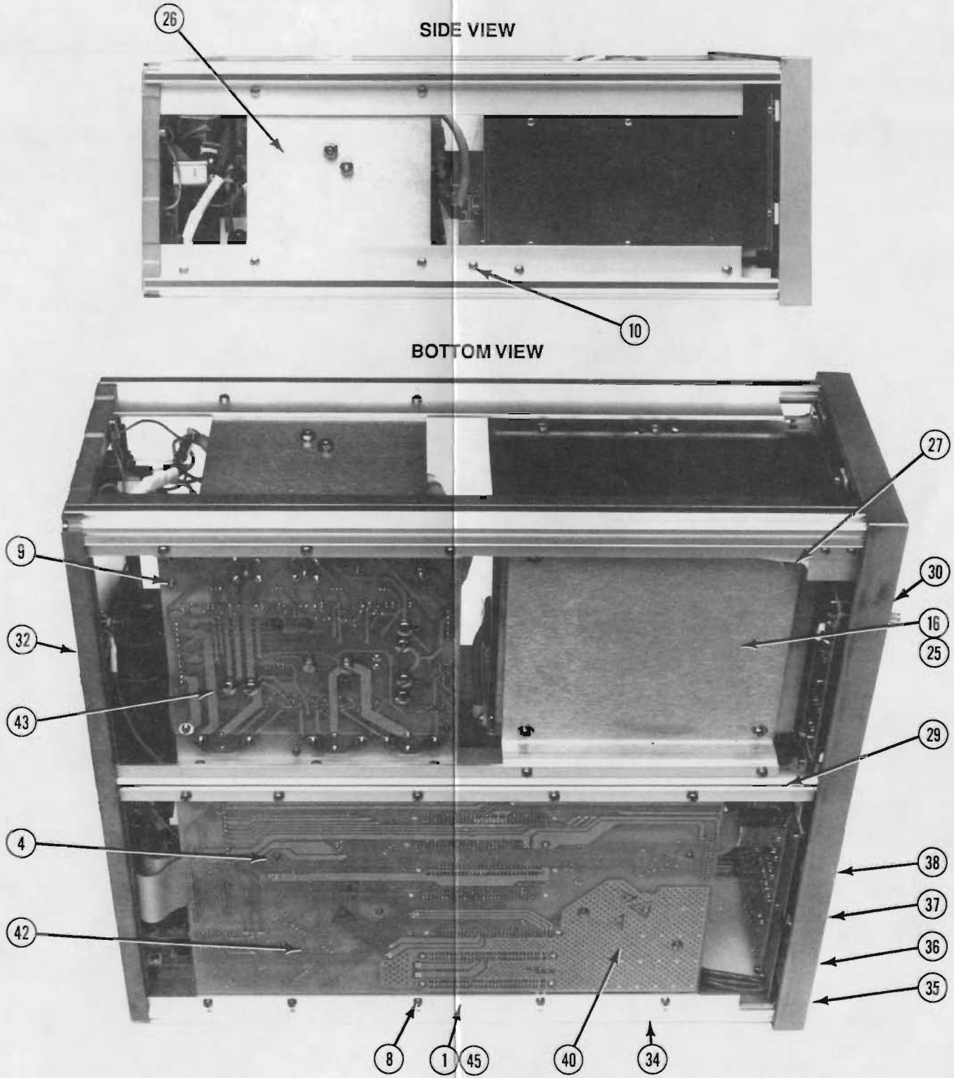
Figure 5-1. Case Assembly 561-D-32501 Sheet 1 of 2
