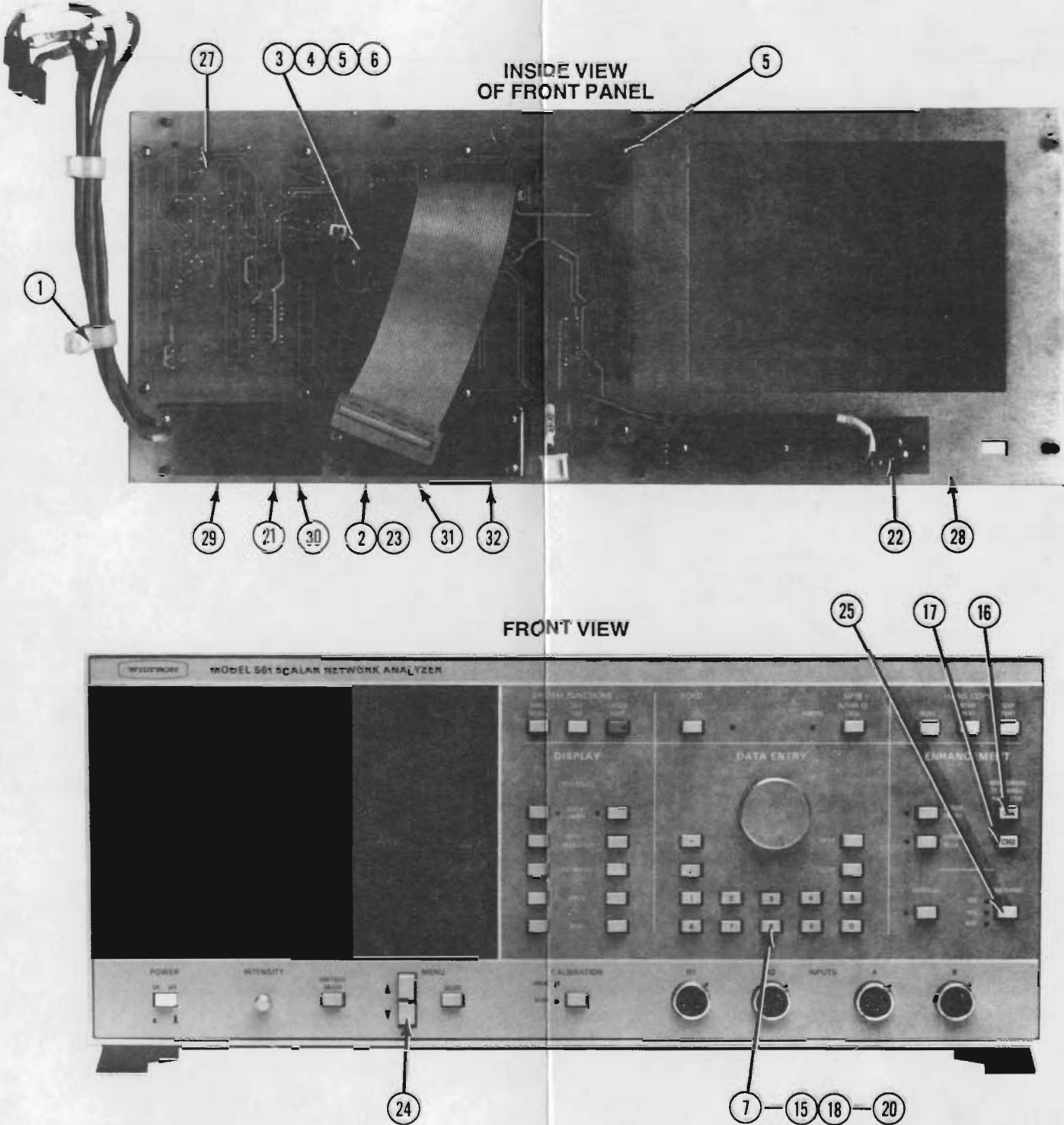
Figure 5-2. Front Panel Assembly 561-D-32502 Sheet 1 of 1
